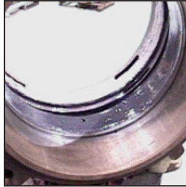
Prepared, coated and protected water jacket
